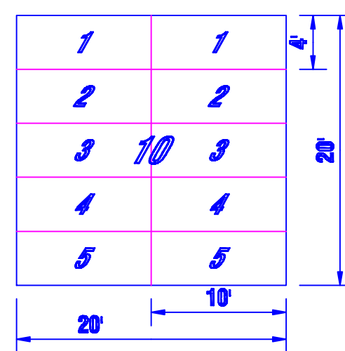
TYPICAL SPACE NUMBERING AND BLOCK DIMENSIONING
